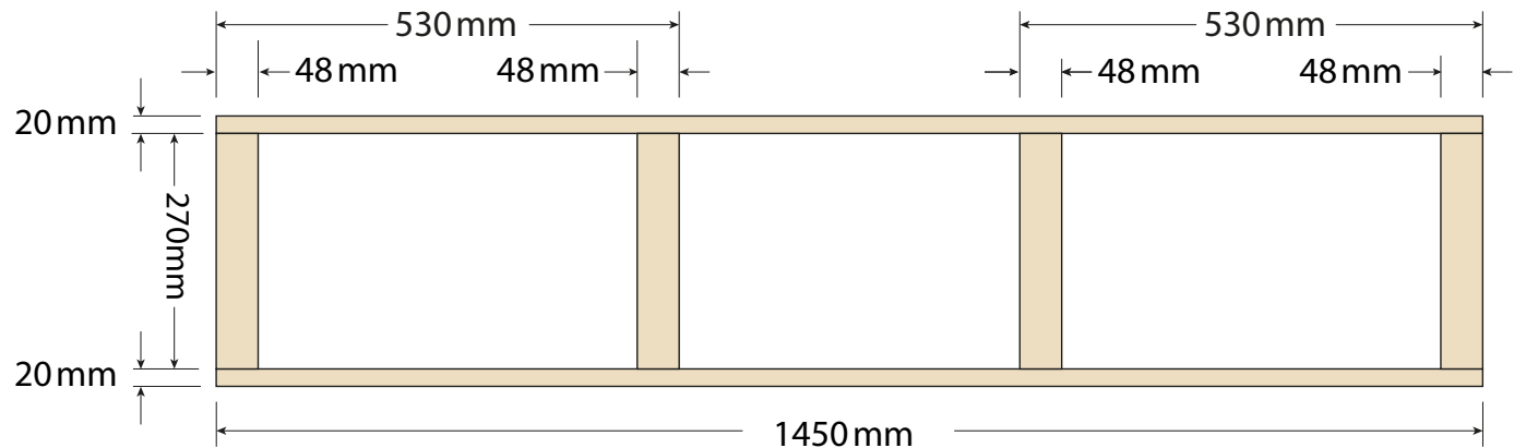
4. Lower Frame
