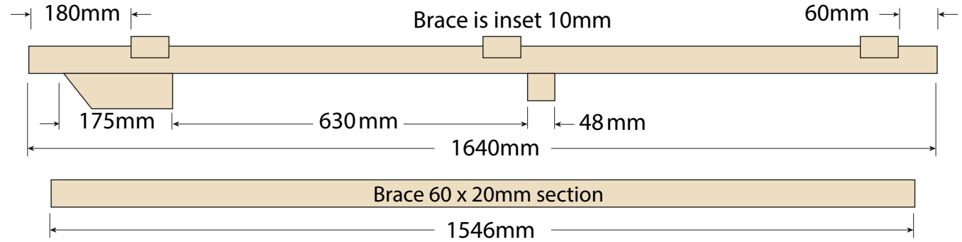
3. Upright Supports
